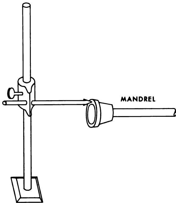
1 FIXED POINTER FOR CHECKING ALINEMENT OF MANDREL COLLAR
